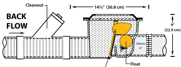
ML-FR4 IN CLOSED POSITION... PREVENTS SEWAGE BACK-FLOW
